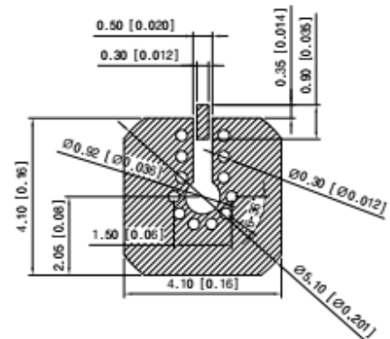
<PC8 Land Pattern>
