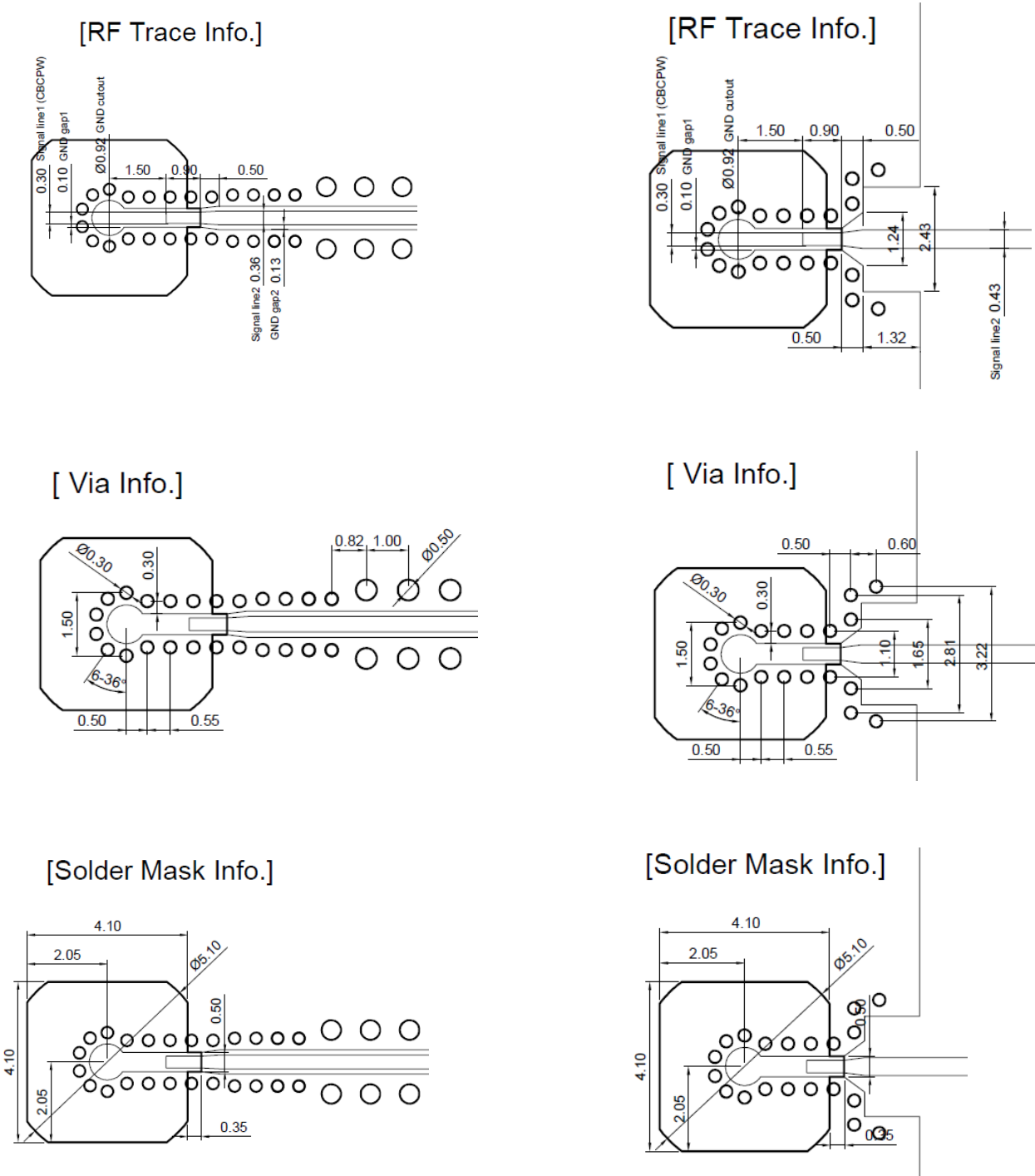
Conductor Backed CPW type
