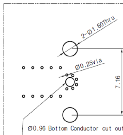
Recommended Bottom PCB Pattern
