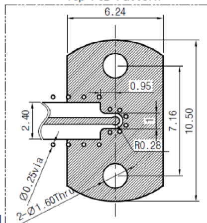
Recommended Top PCB Pattern
